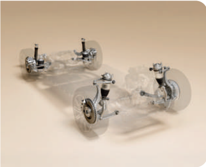
All-aluminum Independent Suspension
